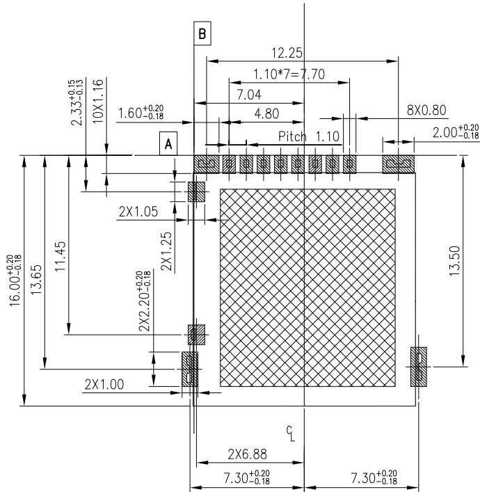
PCB PATTERN LAYOUT (GENERAL TOLERANCE:±0.05)
