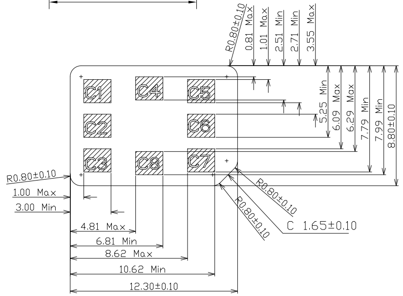
NANO SIM CARD 12.30mm X 8.80mm
