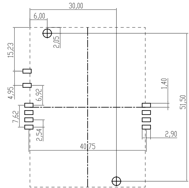
Recommended P.C.B Layout (Top Side) TOL.: ±0.05
